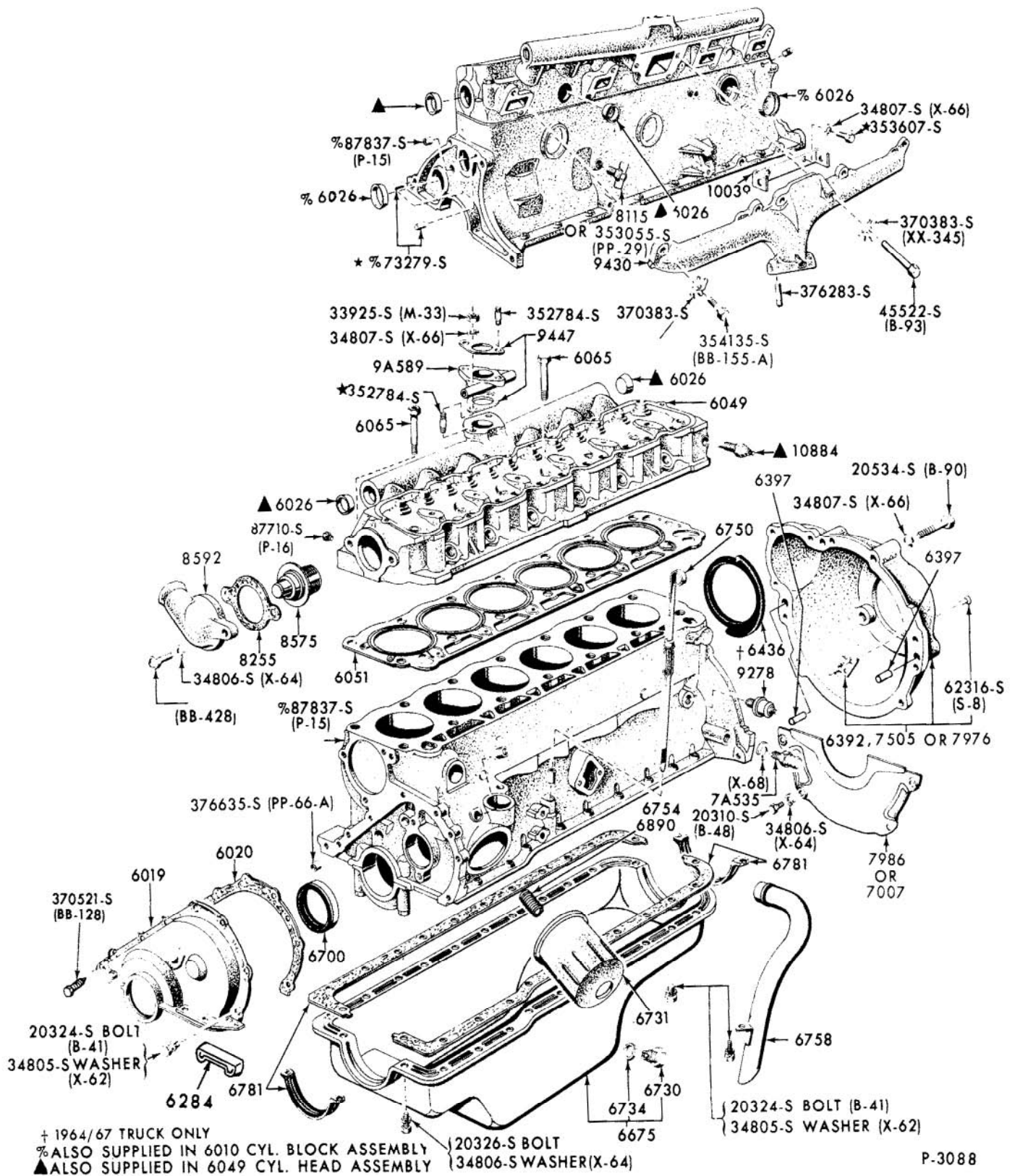
CYLINDER BLOCK AND RELATED PARTS - TYPICAL 1973 6 CYL. 200 AND 250
