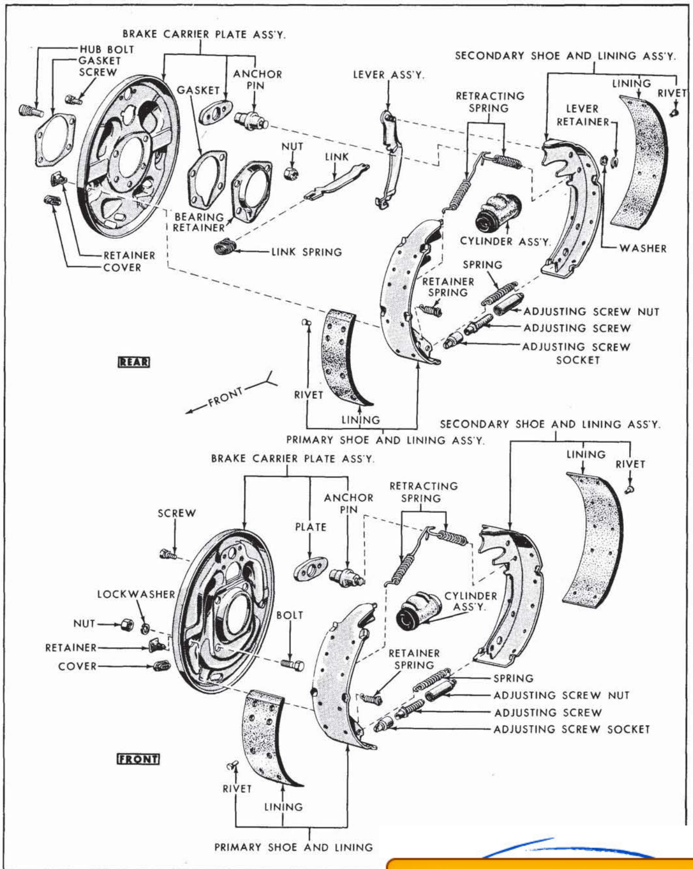
FIG. 1—Front and Rear Brakes—Disass
